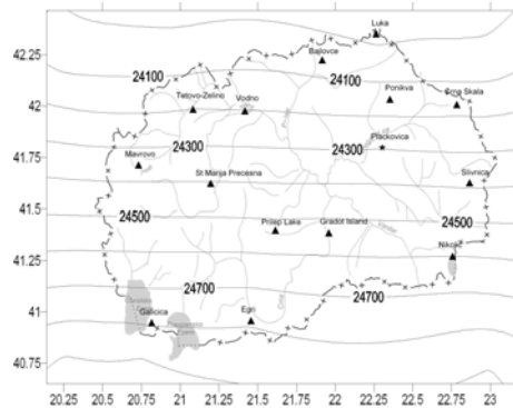
Fig. 4. Map of the horizontal component (H) from the IGRF 2000 model for epoch 2004.5.
