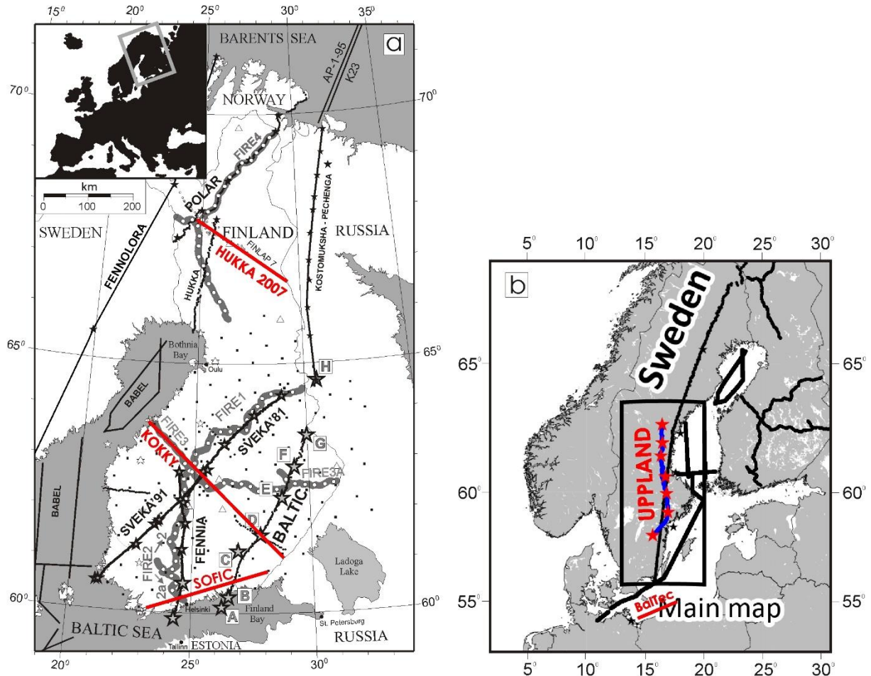
Fig. 7. Location of main onshore and offshore seismic experiments in the Fennoscandia and Baltic Sea: a – SVEKA transect ( SVEKA '81 and SVEKA '91 profiles) BALTIC , POLAR and FENNIA profiles, and deep reflection profiles FIRE 1–4 (modified after Janik et al. 2009). Positions of record stations of the SVEKALAPKO temporary passive array are denoted by rectangles (temporary broadband and short-period stations) and by triangles (permanent stations). Inset map shows the location of target area in Europe. Profiles conducted since 2007 are marked in red (a – HUKKA 2007 , KOKKY , SOFIC , b – UPPLAND and BalTec ). Stars represent the shot points of the profiles; black dots represent recording stations of the DSS experiment; grey dots represent receiver stations; and large white dots represent selected CDP points of the deep seismic reflection experiment FIRE . Additionally, the positions of other DSS profiles in the area ( FENNOLOLA , Kostomuksha–Pechenga and BABEL ) were presented.
