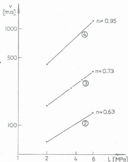
Fig. 6. The velocity of crack propagation as a function of stress load. Curves for different points along the crack path
