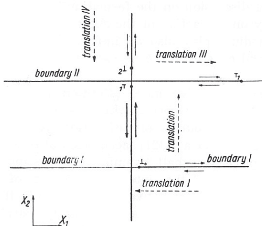
Fig. 7. Crossing mechanism
