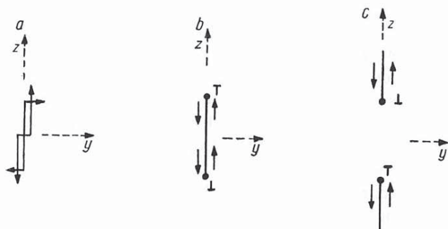
Fig. 10. Model equivalence for finite edge dislocations lying along x -axis: a) dynamic dipole pair, b) equivalent pair creation \top \perp , c) equivalent pair annihilation \perp \top
