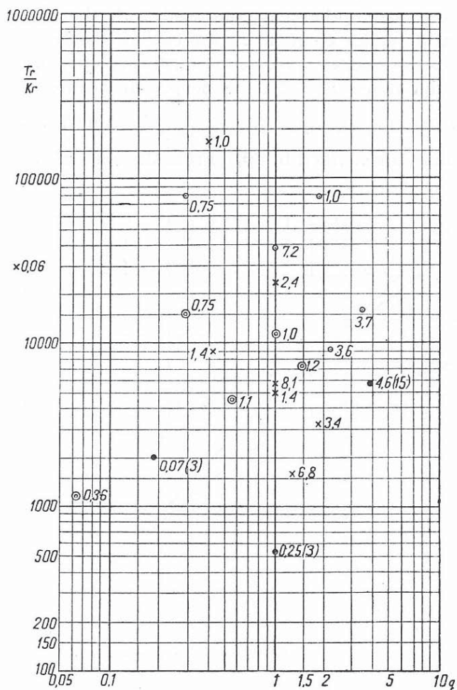
Fig. 21. Observational date: \frac{T_r}{K_r}(q, p)
