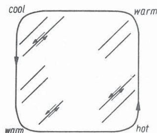
Fig. 1 Equivalence of stresses between thermal convection and dislocation density
