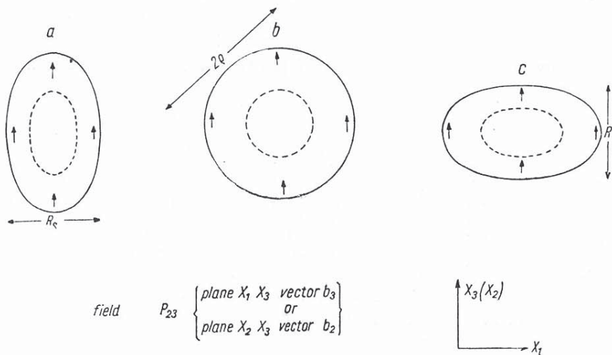
Fig. 2. a) Approach to pair of screw dislocations, b) Loop dislocation, c) Approach to pair of edge dislocations
