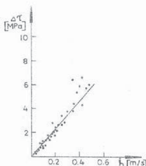
Fig. 7. Stress drop and particle velocity for stick slip (J o h n s o n, 1978)
