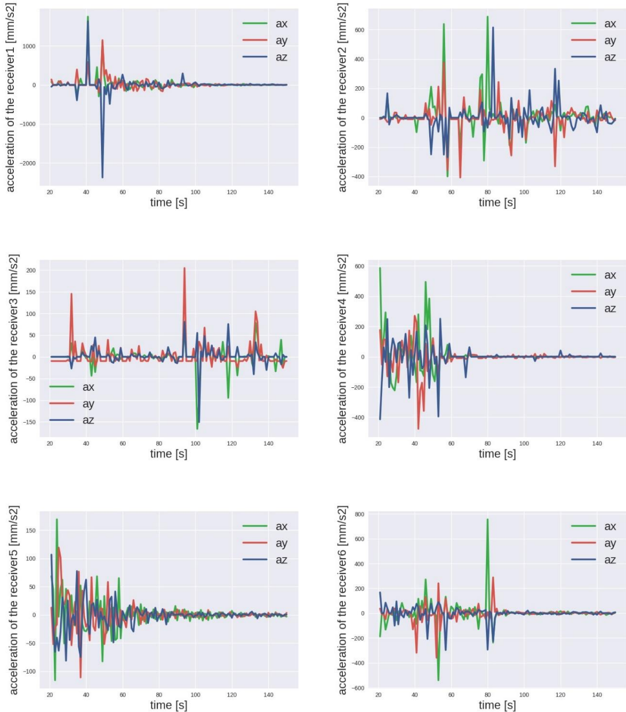
Fig. 56. Simulated acoustic signals generated by 200 \text{ m}^3 of ice falling from the height of 3 m: acceleration readings from receivers 1 to 6 placed in water.
