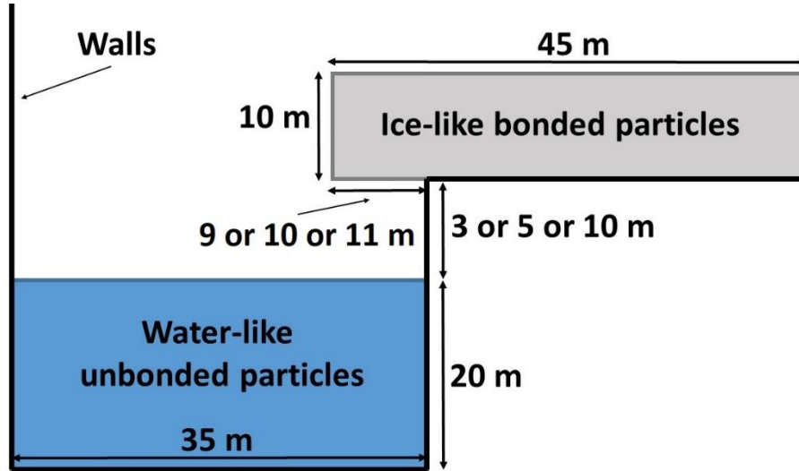
Fig. 51. The 2D cross-section of DEM model of calving glacier.
