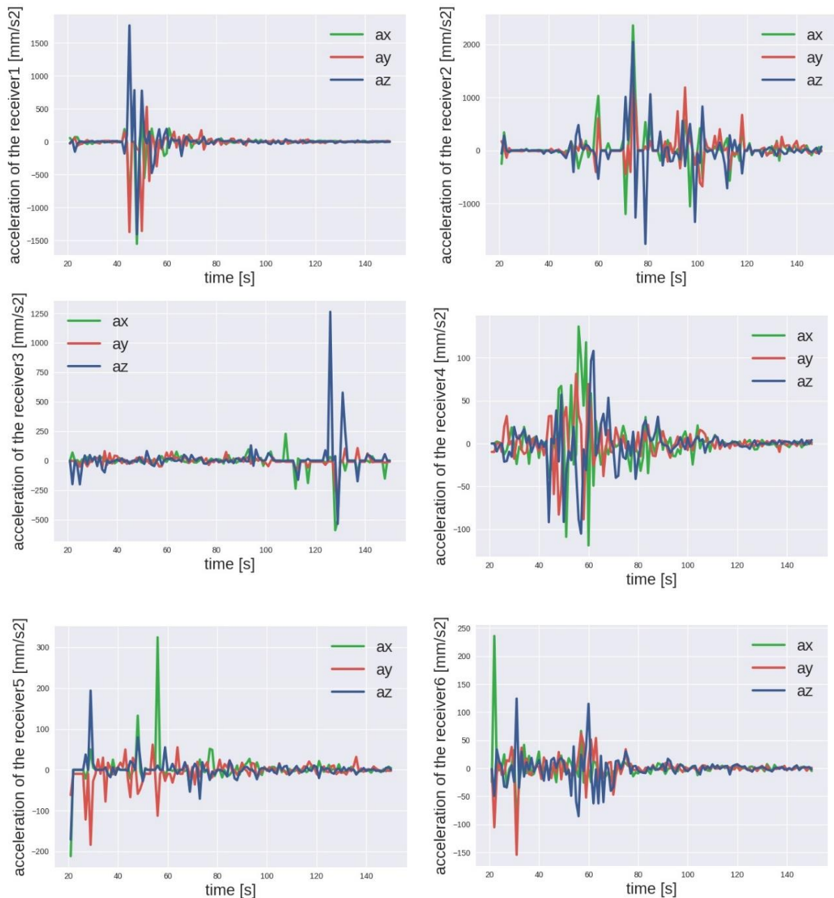
Fig. 58. Simulated acoustic signals generated by 180 m 3 of ice falling from the height of 5 m: acceleration readings from receivers 1 to 6 placed in water.
