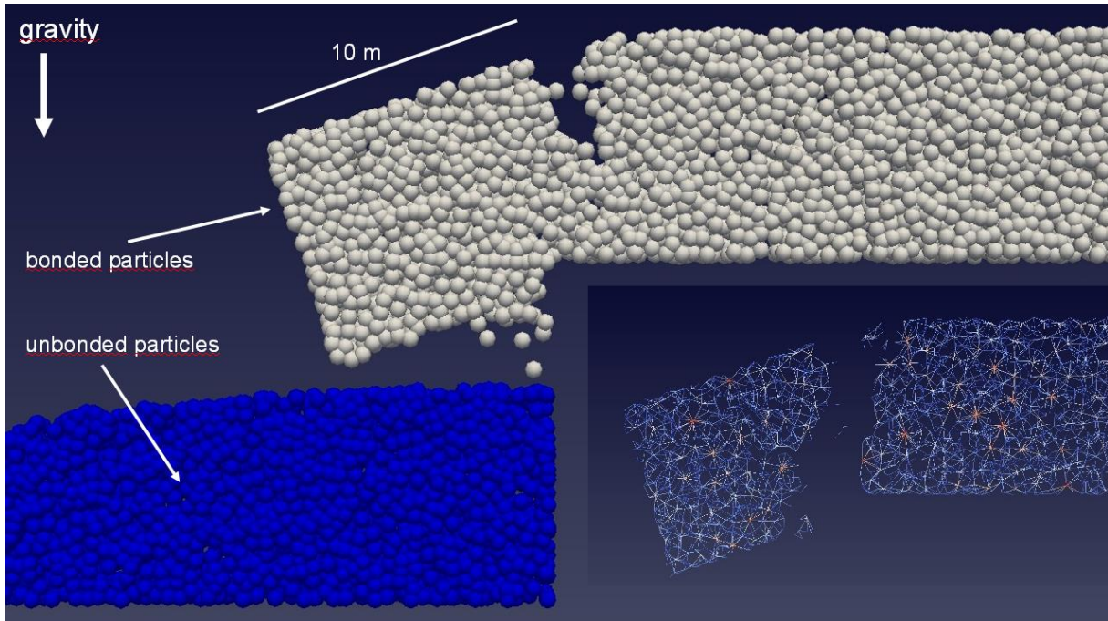
Fig. 52. Part of the glacier goes down due to gravity force – a snapshot from the simulation. In the right bottom corner – a view of breaking bonds.
