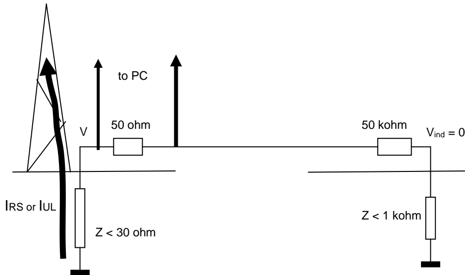
Fig. 2. Set-up for measuring a “loop voltage” during a direct lightning strike (return stroke current I_{RS} ) or an upward leader (current I_{UL} ) from the tower. Input resistor at the PC is 50 ohm, while the resistor on the other end of the coaxial line, at the independent ground point is 50 k ohm. V is a potential of the grounding system of the installation. The arrow shows the direction of positive charges flowing in the return stroke or upward leader.
