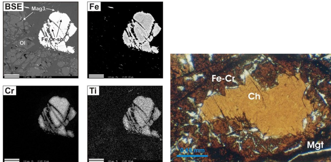
Fig. 1. BSE-SEM maps for chromite grains from chromite ore (JGSM, Tapadla, ferri-chromite).
