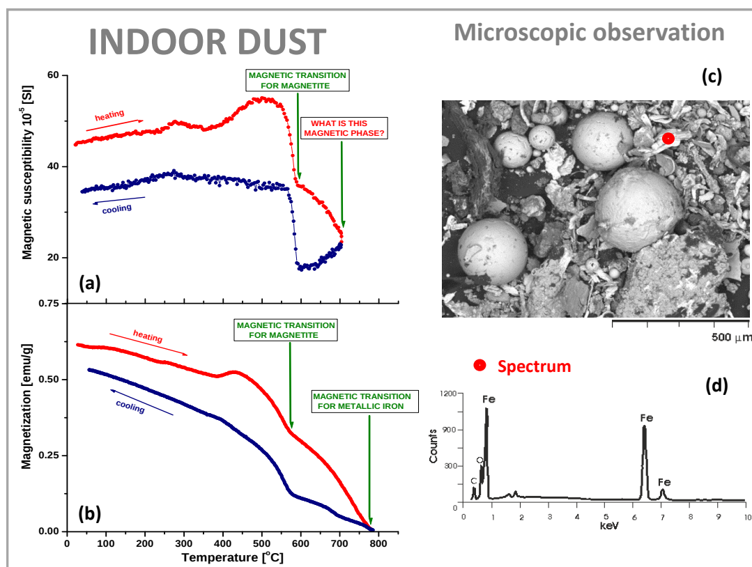
Fig. 1. Temperature changes of magnetic susceptibility \chi(T) in the temperature range of 30–700°C (a), changes of induced magnetization M(T) in the temperature range of 30–800°C (b), electron scanning microscopy observation (c), energy-dispersive X-ray spectra (d).
