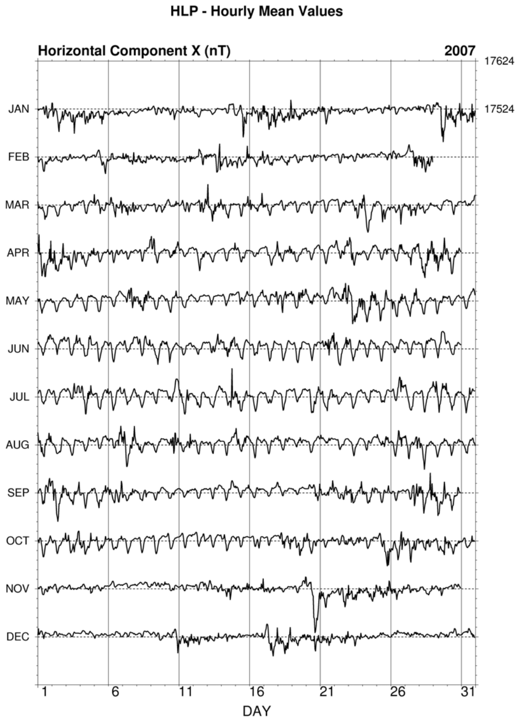
Fig. 21. Hourly mean data plot of X component for Hel 2007.
