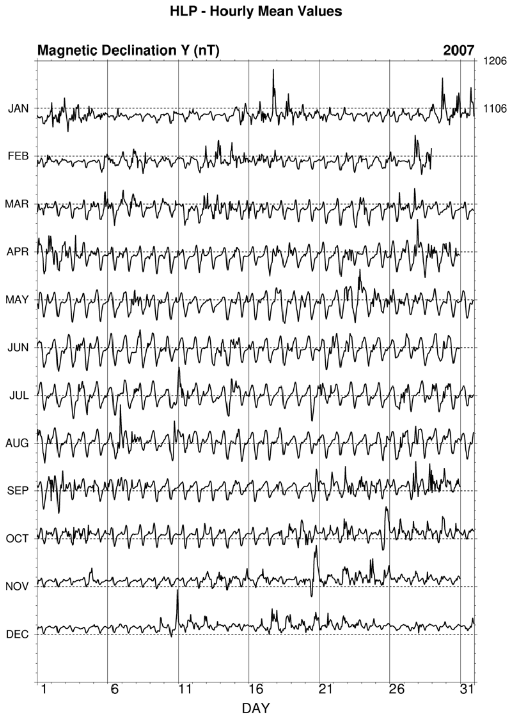
Fig. 22. Hourly mean data plot of Y component for Hel 2007.
