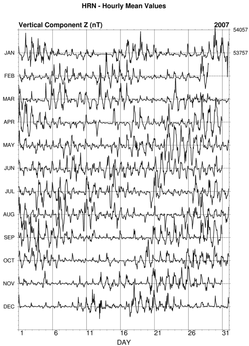
Fig. 31. Hourly mean data plot of Z component for Hornsund.
