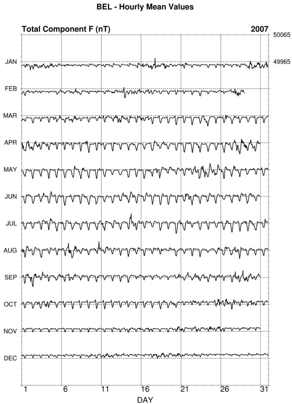
Fig. 16. Hourly mean data plot of F component for Belsk 2007.
