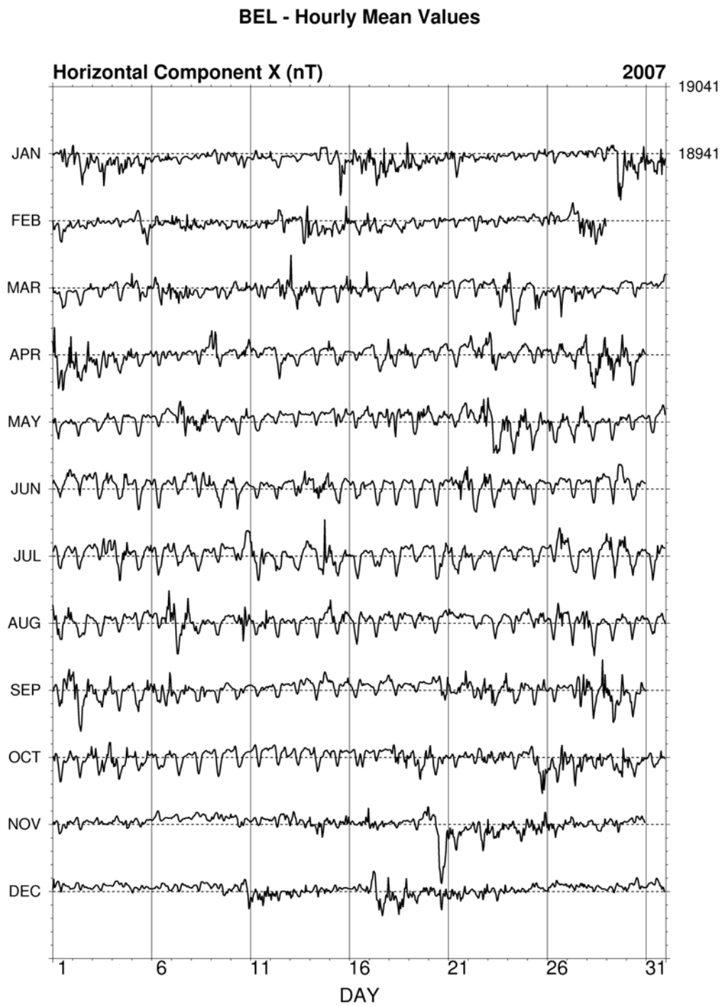
Fig. 13. Hourly mean data plot of X component for Belsk 2007.
