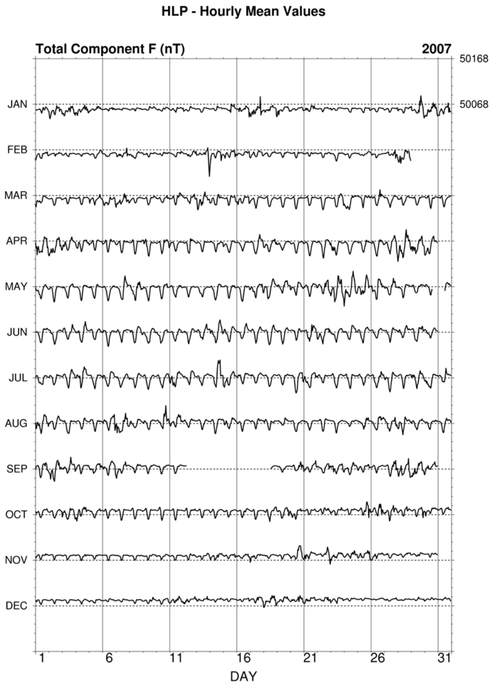
Fig. 24. Hourly mean data plot of F component for Hel 2007.
