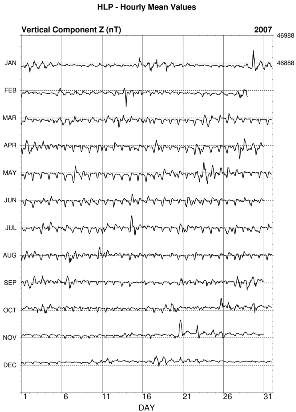
Fig. 23. Hourly mean data plot of Z component for Hel 2007.
