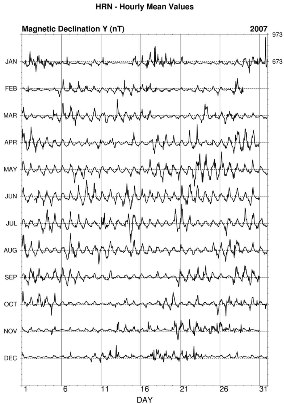
Fig. 30. Hourly mean data plot of Y component for Hornsund.
