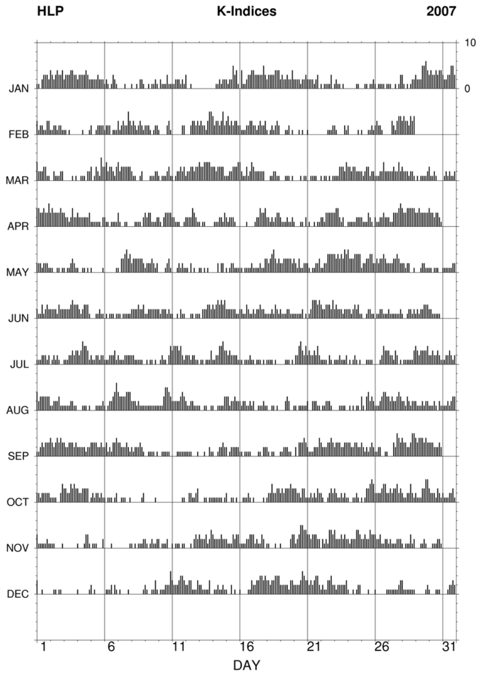
Fig. 19. K-indices in graphical form, Hel 2007.
