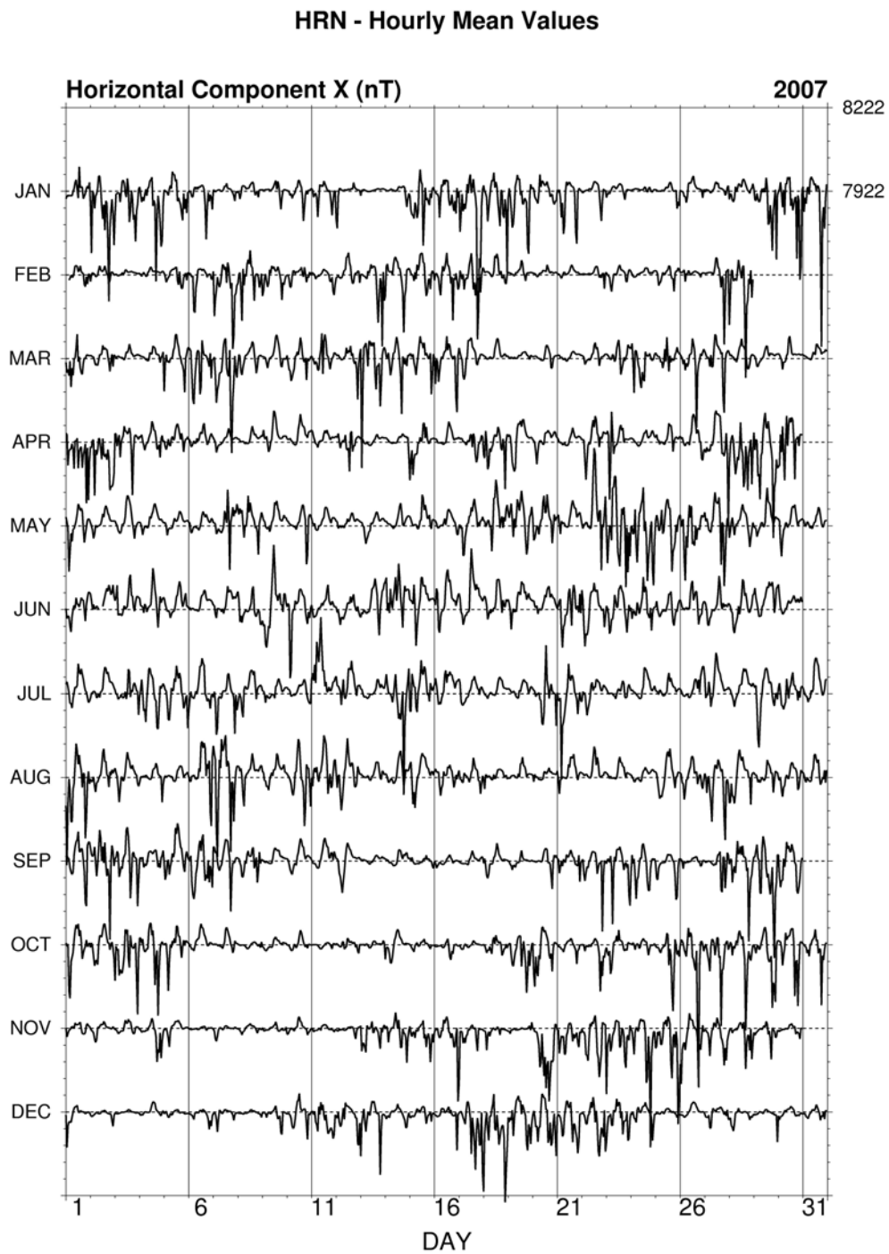
Fig. 29. Hourly mean data plot of X component for Hornsund.
