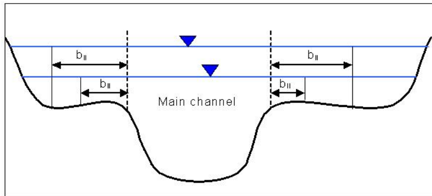
Fig. 2. Determining the range of active cross-section.
