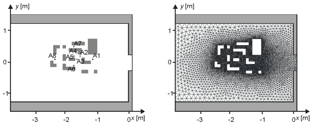
Fig. 3. Model city configuration, gauging points location (left) and part of numerical mesh (right).
