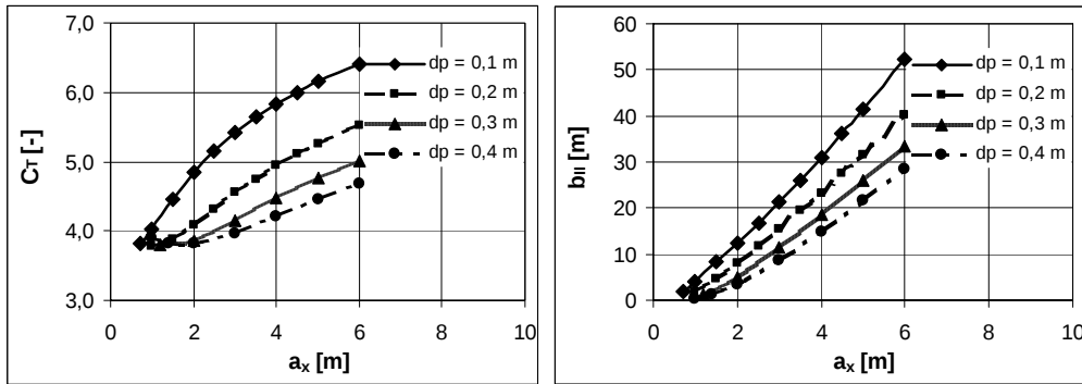
Fig. 2. C_T and width of b_H as a function of tree diameter and the span between trees.
