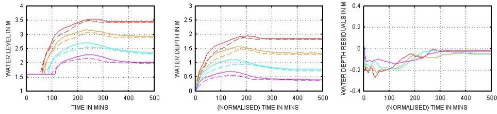
Fig. 5. Reparameterisation of the time series (left) to the arrival time of the flood wave (centre). Solid lines: CGM results. Dashed lines: FGM results. The colours represent different values of q .
