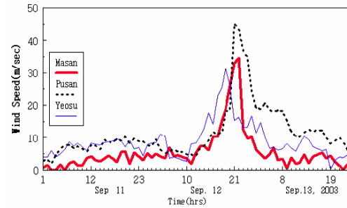
Fig. 3. Wind speed in Masan, Pusan and Yeosu.
