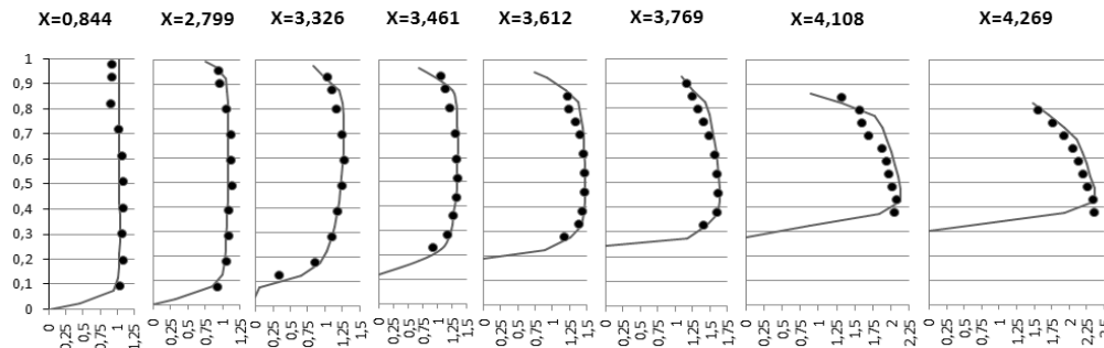
Fig. 5. Comparison of distributions of horizontal velocity components: ~ calculations and • measurements.
