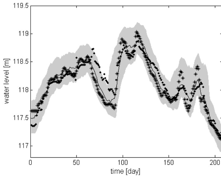
Fig. 4. Validation of the STF simulator for the cross-section at Suraz; dots denote observations, stars denote UNET simulations and continuous line denotes the simulator estimates with 0.95 confidence bounds shown by shaded area.
