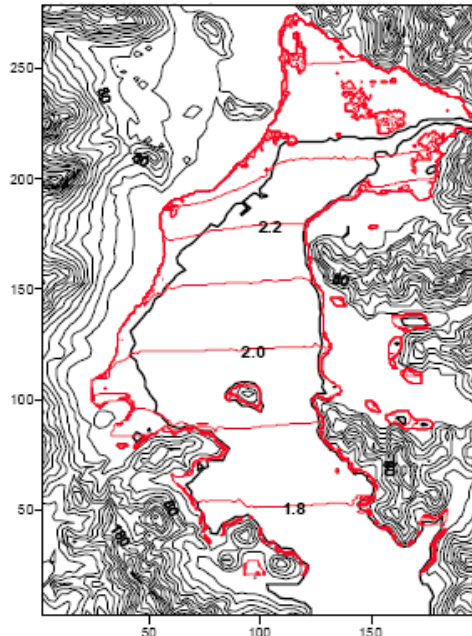
Fig. 9. Computed inundation area (red line).
