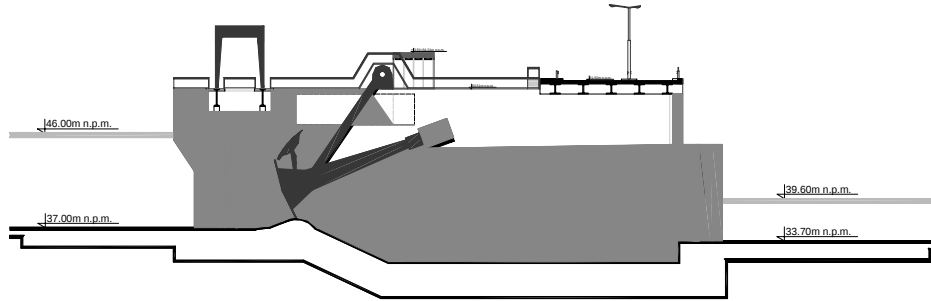
Fig. 3a. Characteristic cross-section of weir 'Nieszawa' span.
