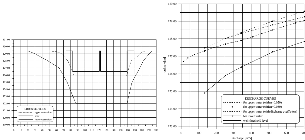
Fig. 2b. Calculation scheme of cross-sections and results of calculations for object ‘Bukówka’.
