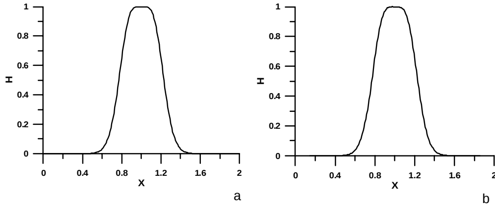
Fig. 3. Result of modeling of scalar field rotation using simple upstream differencing scheme: a) in Cartesian coordinates; b) in curvilinear coordinates.
