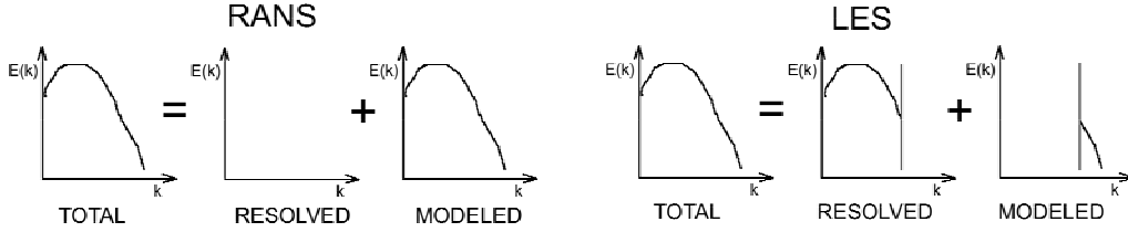
Fig. 1. Decomposition of turbulent energy spectra ( E(k) ) in RANS and LES, k is the wave number, i.e. inverse characteristic length of objects. Adopted from (Sagaut 1998).
