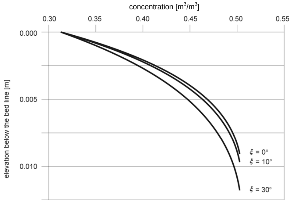
Fig. 2. Concentration profiles for different river bed slopes ( d = 0.4 mm, u_f = 0.12 m/s).
