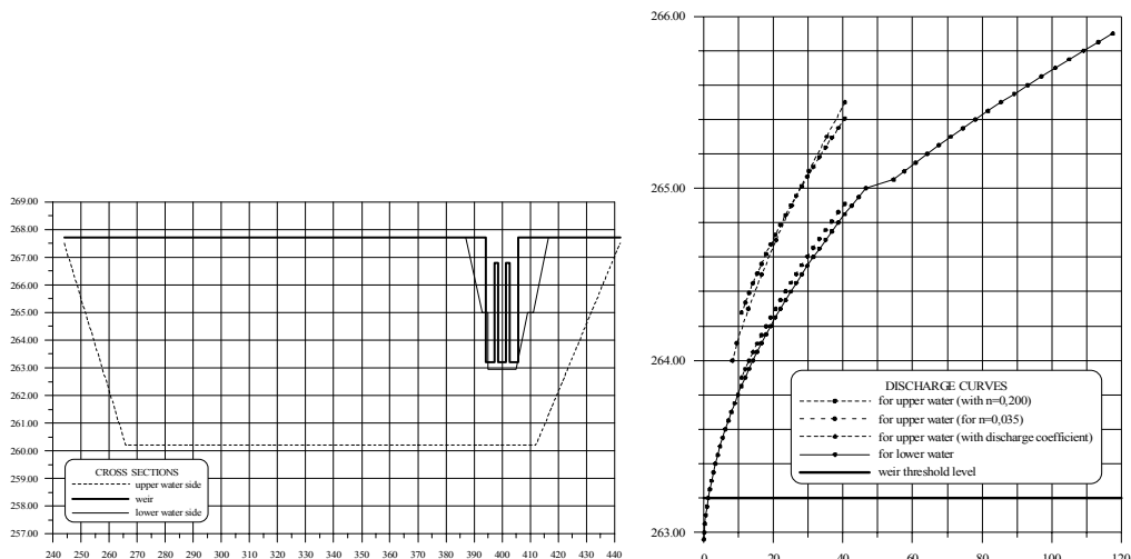
Fig. 1b. Scheme of calculation the cross-sections and results of calculations for object ‘Kuznica Warężyńska’.
