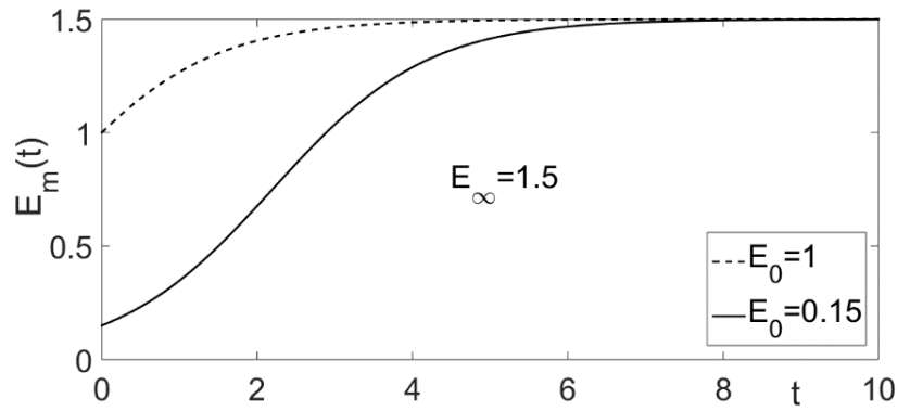
Fig. 1. Saturation of the magnetic energy of a force free mode for two cases: E_\infty/E_0 = 10 (solid line) and E_\infty/E_0 = 1.5 (dashed line); in both cases the asymptotic energy value is E_\infty = 1.5 , but the initial energies differ (after Mizerski 2020).
