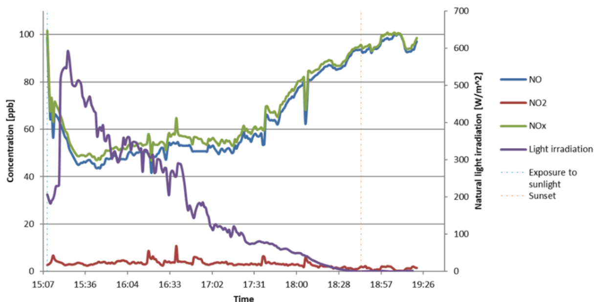
Fig. 2. NO, NO 2 and NO x abatement with natural UV irradiance measured with the novel test method. Figure from Witkowski et al. (2020).
