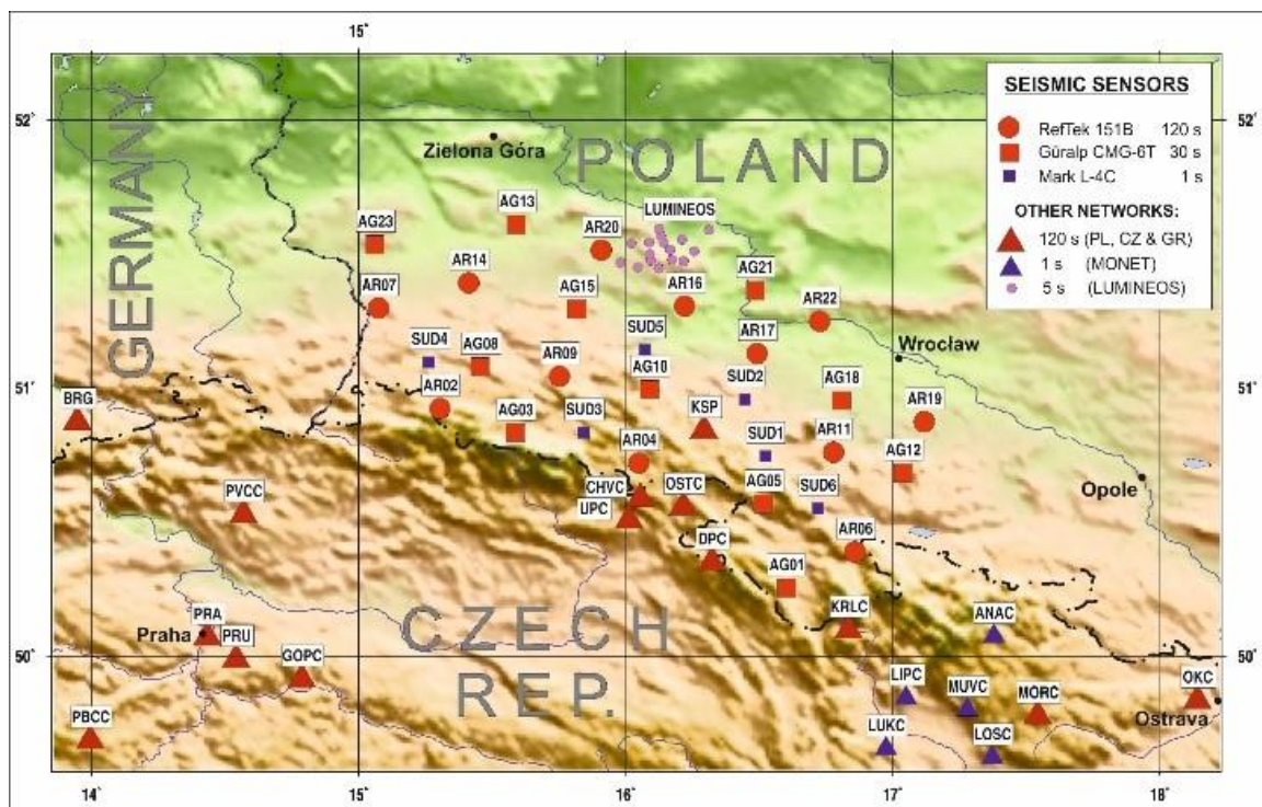
Fig. 1. Location of the seismic stations of the AniMaLS experiment in the Sudetes. Circles and squares – portable stations, triangles – permanent stations.
