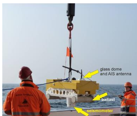
Fig. 1. The Guralp ocean bottom seismometer station. Principal parts are indicated.
