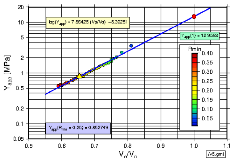
Fig. 2. Scaling of the young modulus with respect to the numerical porosity - the ratio of the volume occupied by particles to the volume of the sample.
