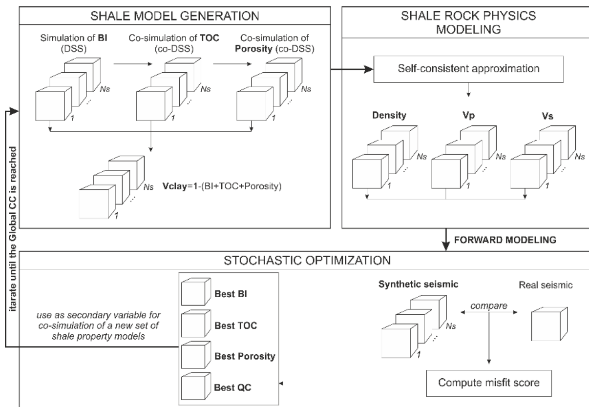
Fig. 1. Schematic representation of the geostatistical shale rock physics seismic AVA inversion methodology (after Cyz and Azevedo 2021).
