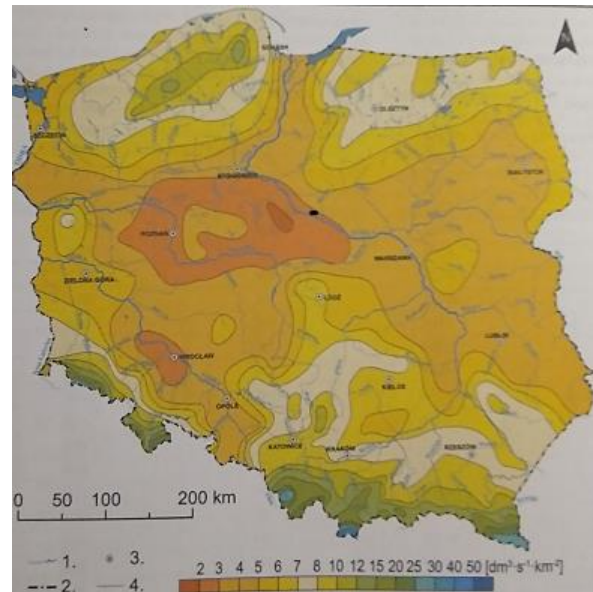
Fig. 9. The runoff module (dm 3 s -1 km -2 ) in Poland.
