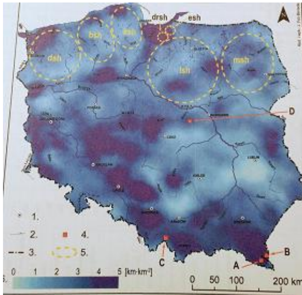
Fig. 8. River network density (km/km 2 ).
