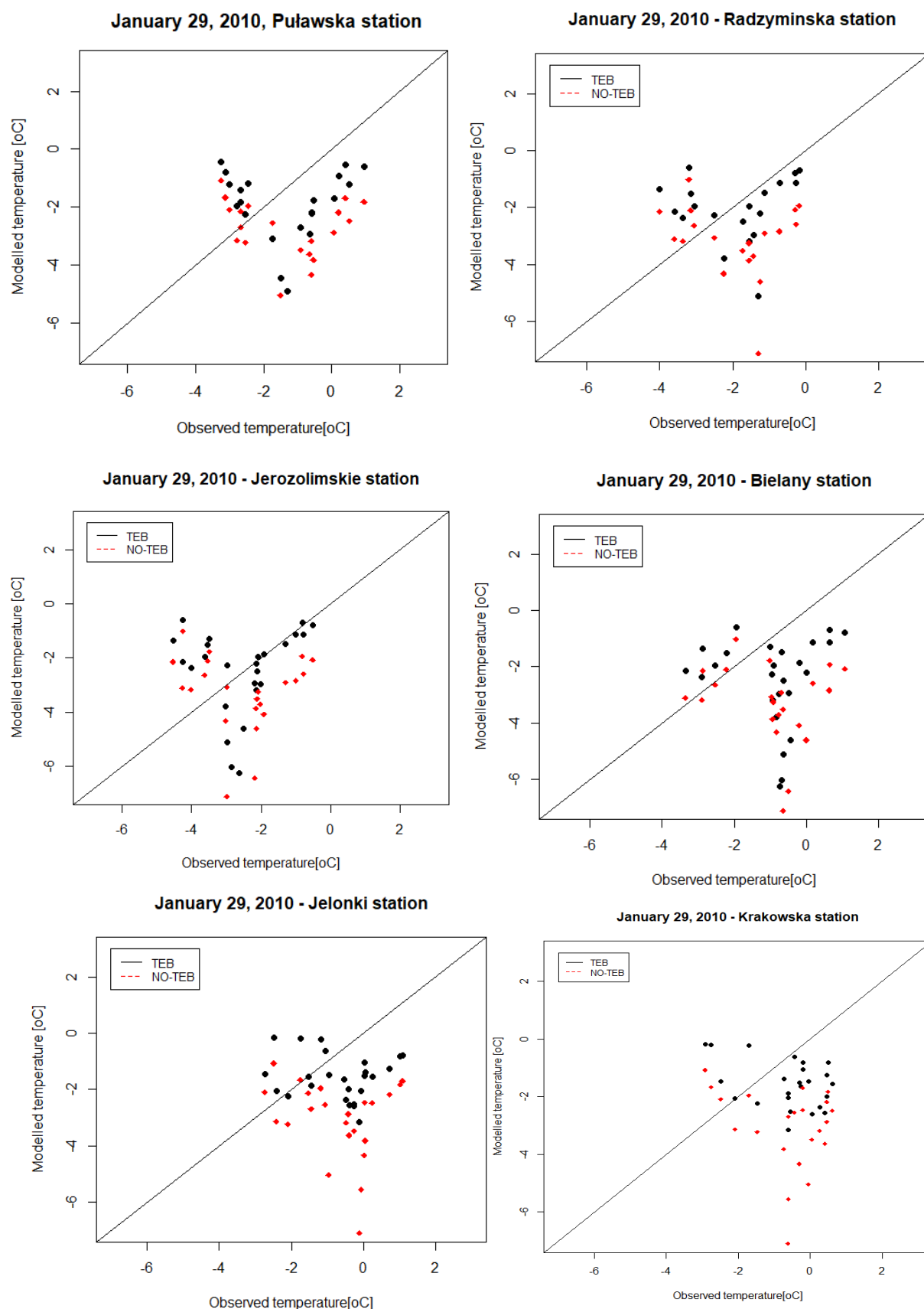
Fig. 56. Near-surface temperature measured at Puławska, Radzimińska, Jerozolimskie, Bielany, Jelonki, and Krakowska stations and calculated by the GEM model for January 29, 2010.
