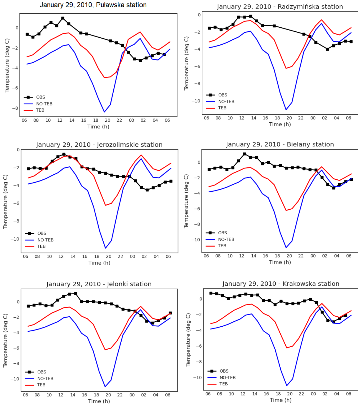
Fig. 52. Comparison of modelled temperature with observations for Puławska, Radzyńska, Jerozolimskie, Bielany, Jelonki, and Krakowska stations for January 29, 2010.
