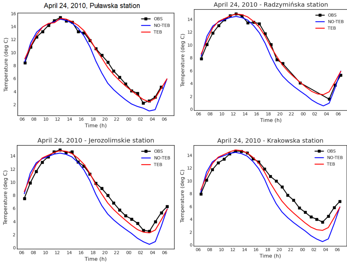
Fig. 53. Comparison of modelled temperature with observations for Puławska, Radzymińska, Jerozolimskie, and Krakowska stations for April 24, 2010.
