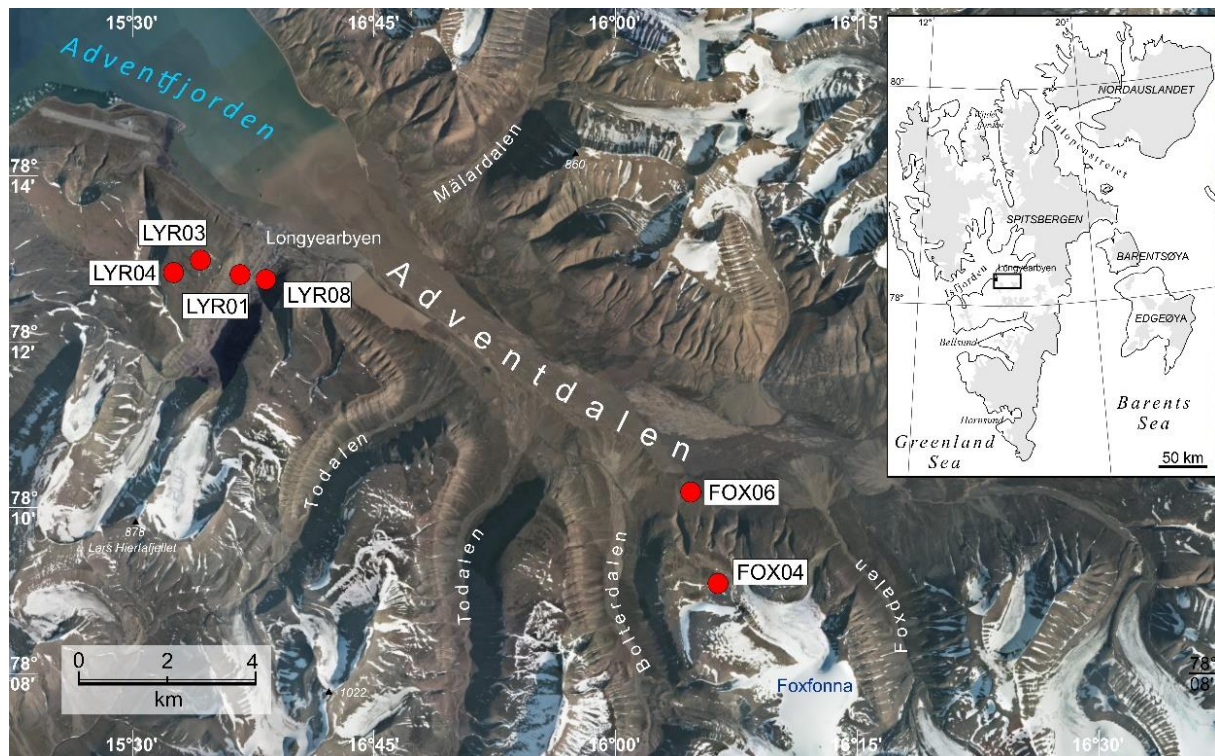
Fig. 1. Location of the study sites in Central Spitsbergen, Svalbard.
